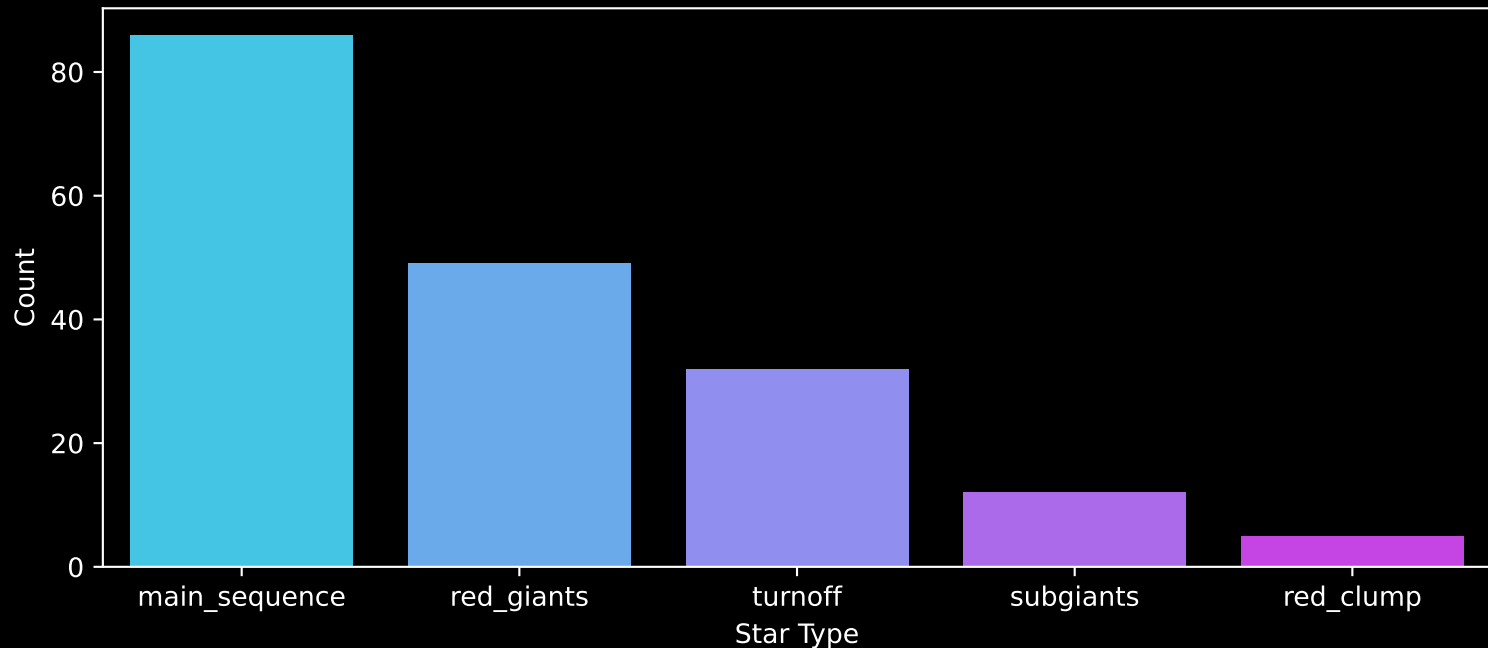
APOGEE DR17 Field: [173+30_MGA] Count plot of Star Type
