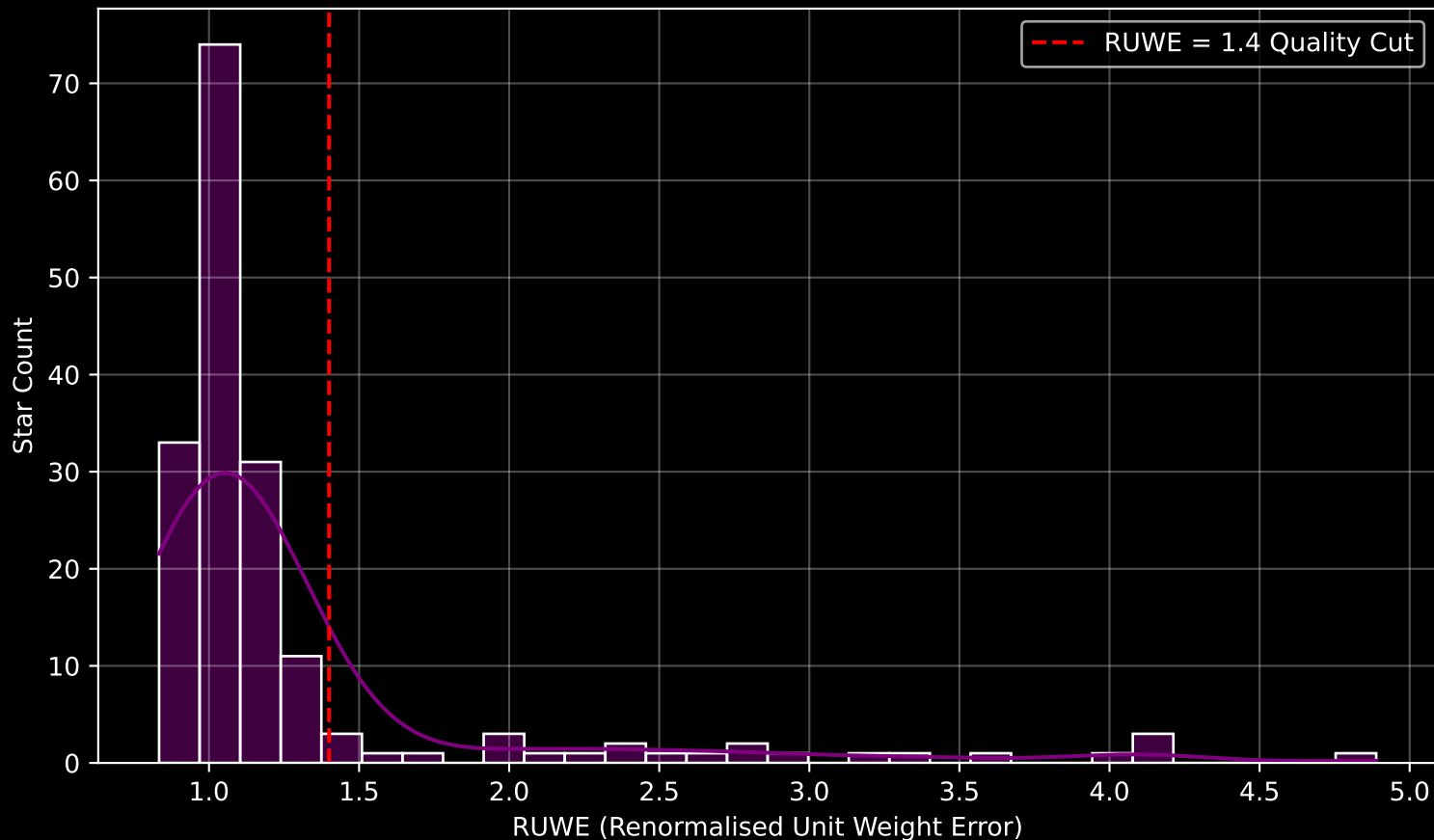
GAPOGEE DR17 Field [173+30_MGA] RUWE Distribution (n= 174)
