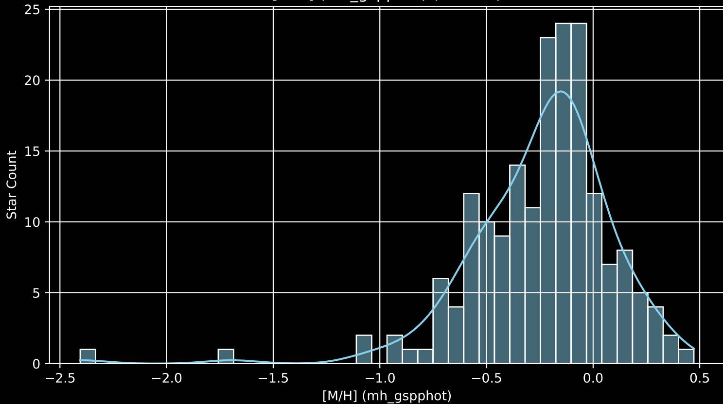
APOGEE DR17 Field: [173+30_MGA [M/H] (mh_gspphot) (n= 184)
