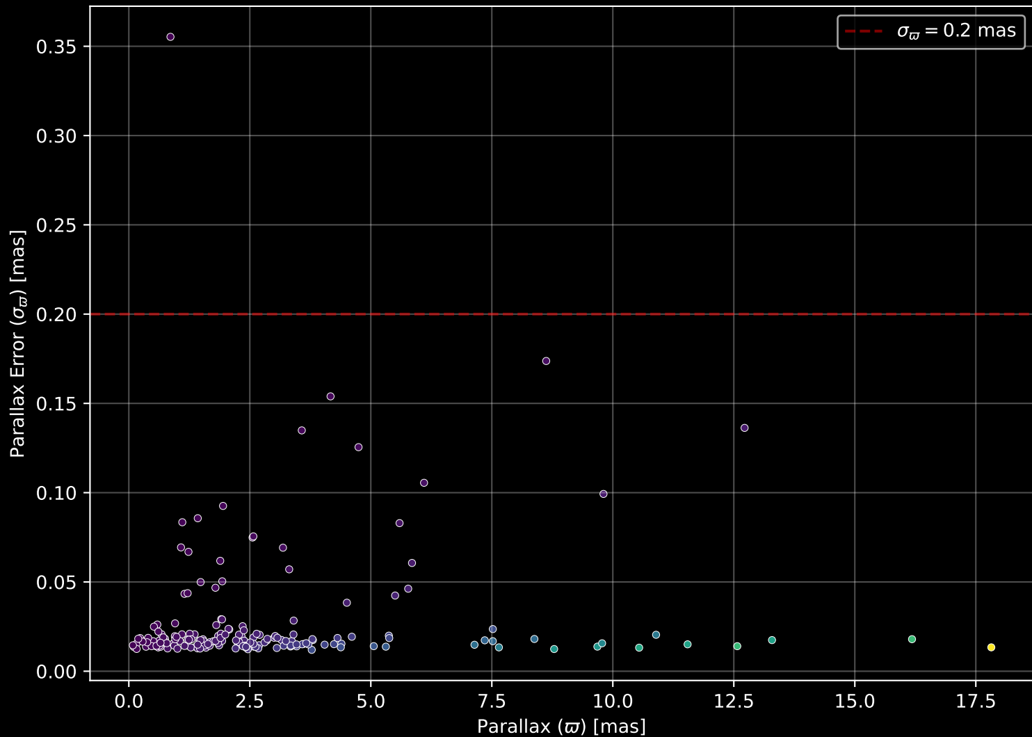
APOGEE DR17 Field: [173+30_MGA] Parallax Quality (n= 184)
