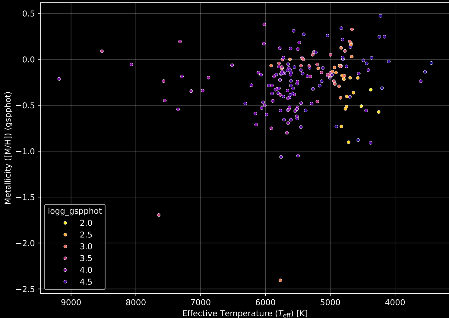
APOGEE DR17 Field: [173+30_MGA] Stellar Population Parameters (n= 184)
