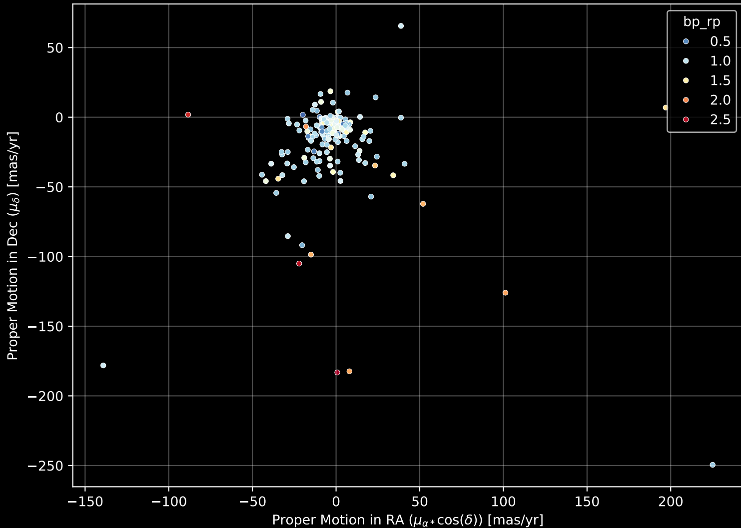
APOGEE DR17 Field: [173+30_MGA] Proper Motion Diagram (n= 184)
